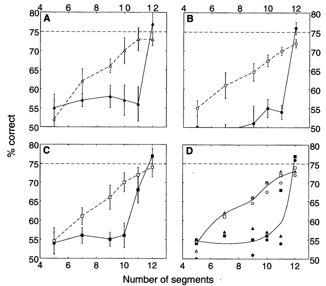
FIG. 4. Contour detection performance as a function of the number of segments (results corresponding to Fig. 3). Gap size was \Delta_o for jagged contours and \Delta_c for circular contours. (A–C) Individual performance curves of three observers (triangles, FP; circles, IK; squares, HM). Open symbols represent performance for jagged contours, closed symbols for circular contours. (D) Averaged result for the three observers. Performance increased continuously from chance level to threshold for nonclosed jagged contours. For circular contours performance stayed at chance level, and threshold performance occurred only when the contour was closed or nearly closed (11–12 presented elements).
