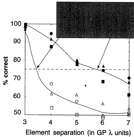
FIG. 2. Psychophysical results corresponding to Fig. 1. Percent correct performance for the detection of curved contours was measured as a function of distance between neighboring elements in a 2AFC paradigm. Results of three subjects (triangles, FP; circles, IK; squares, HM) are shown. Targets were presented on a 16^\circ \times 16^\circ field containing 2000 randomly placed GPs. Target contours were built up from 19–23 GPs (giving rise to the maximal length across the field with all different displacements) of the same parameters as background, having \pm 30^\circ relative angular difference between neighbors. Center of gravity of the lines was randomized around the center of the field in a 1^\circ range. Stimulus duration was 160 msec. Detection of the stacked line at 75% correct response defined \Delta . \Delta_o (open symbols) was 3.3 times the wavelength of the patches (open symbols). \Delta_c (closed contours) was 6 times the wavelength (closed symbols). (Insets) \Delta_o and \Delta_c separation.
